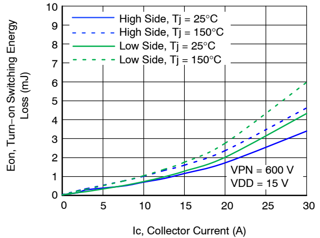
Figure 14. Typ. Turn-on Switching Energy Loss
