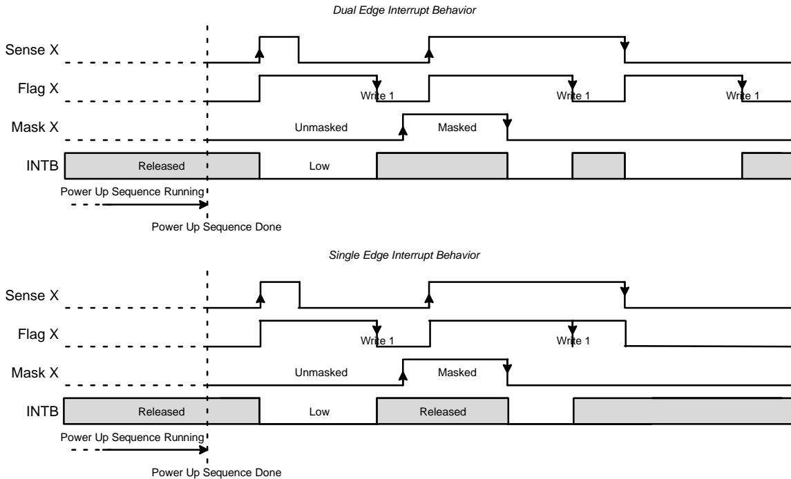
Figure 21. Interrupt Behavior
