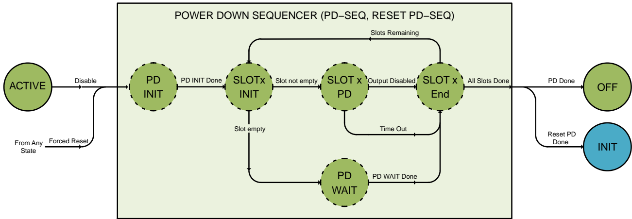
Figure 20. Power Down Sequence State Machine
