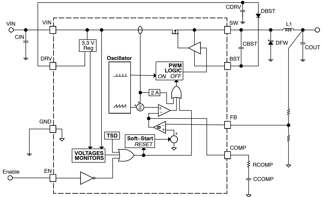
Figure 2. NCV890200 Block Diagram
