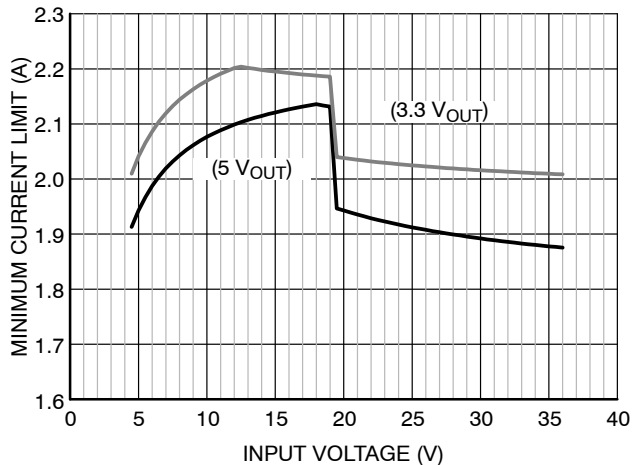
Figure 26. NCV890200 Load Current Capability with 4.7 \mu H Inductor
