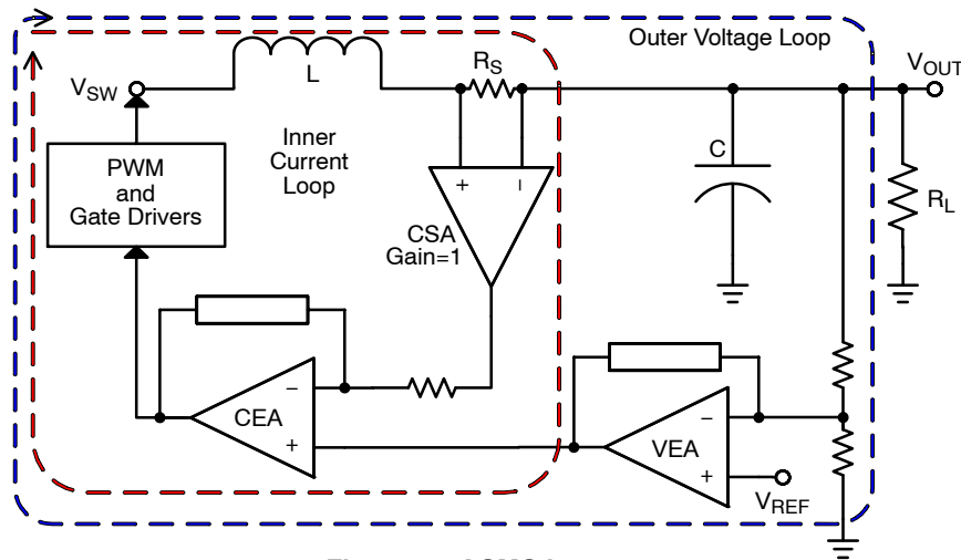
Figure 18. ACMC Loops
