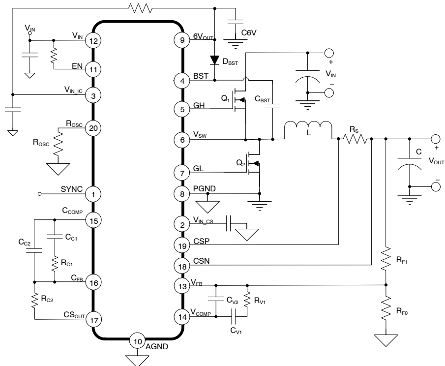
Figure 2. Application Schematic
