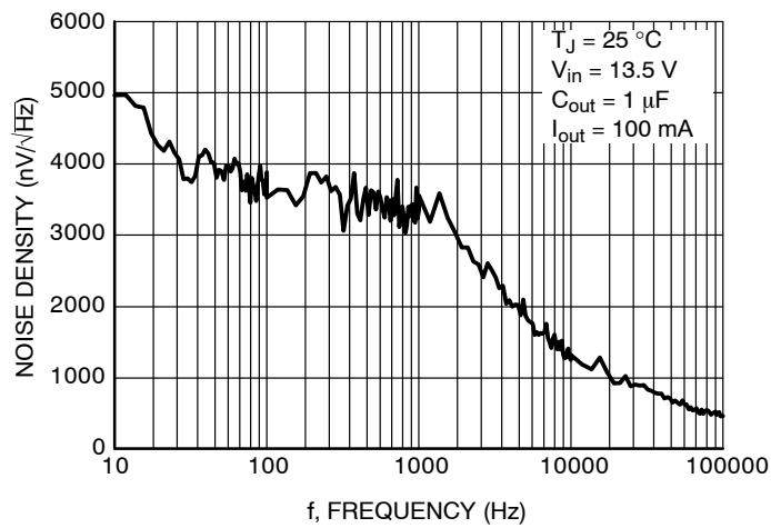
Figure 27. Noise vs. Frequency
