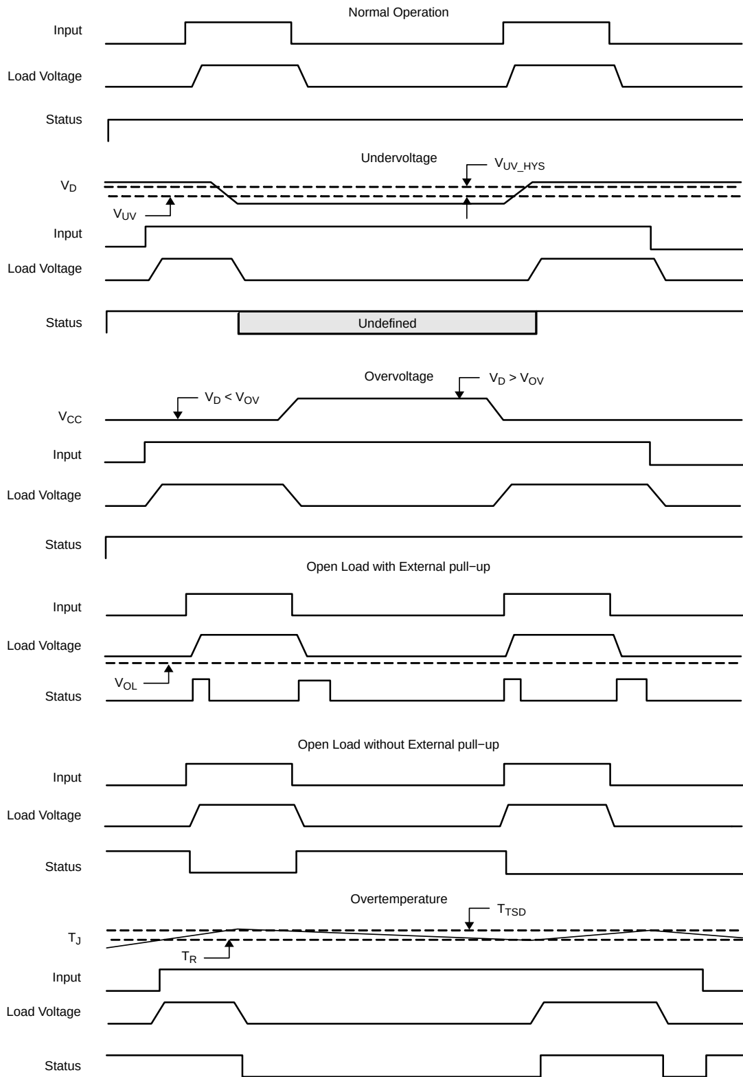
Figure 30. Waveforms
