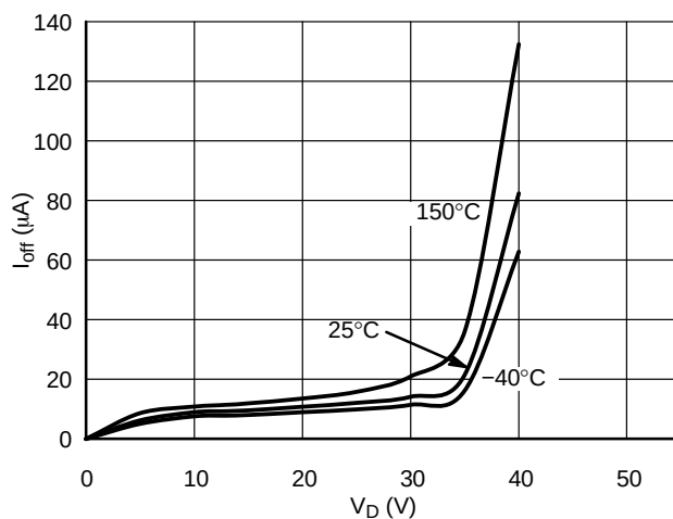
Figure 8. OFF State Standby Current vs. V D
