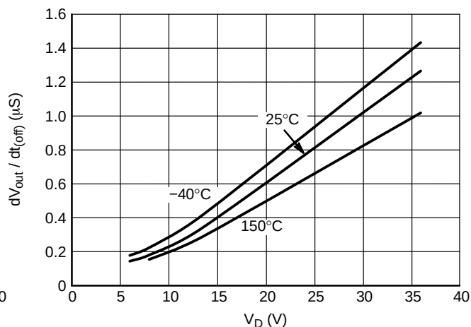
Figure 18. Slew Rate OFF vs. V_D
