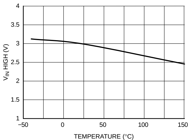
Figure 10. V in Threshold High vs. Temperature
