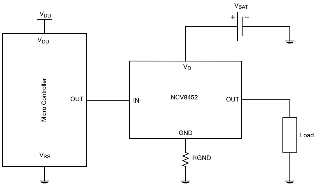
Figure 3. Application Diagram
