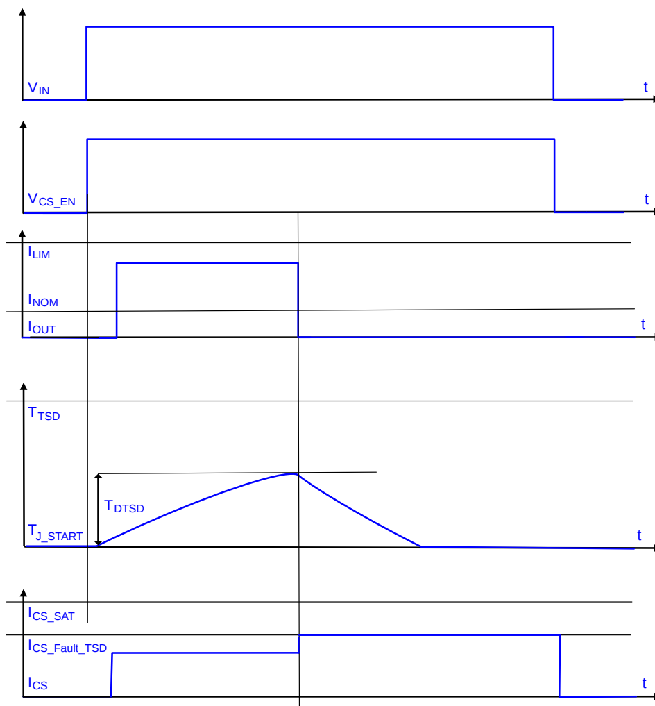
Figure 17. Over-Temperature Protection
