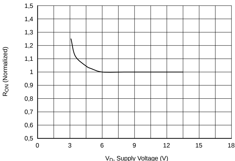
Figure 6. ON-state Resistance
