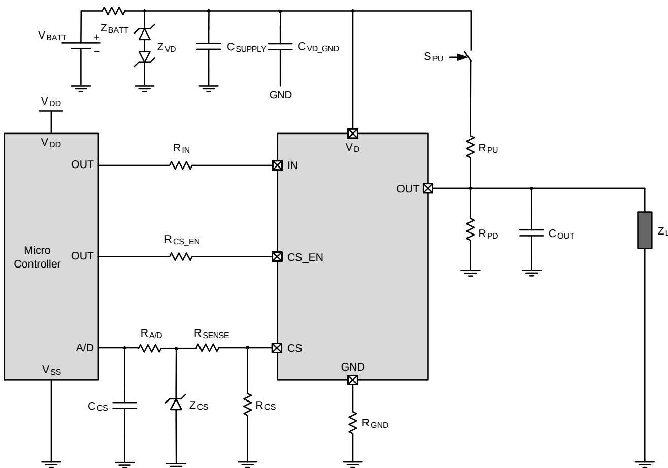
Figure 4. Application Diagram
