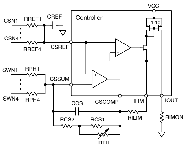
Figure 9. Total Current Summing Amplifier
