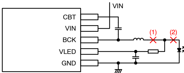
Figure 21. OPENLED Failure
