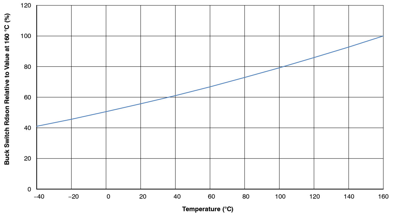
Figure 8. Typical Temperature Behavior of Buck HS Switch R_{ds(on)} Relative to the Value at 160 °C
