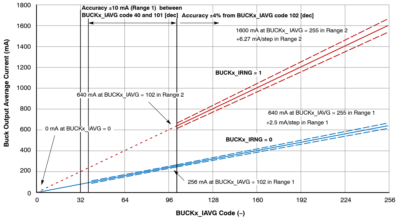
Figure 7. Typical LED Current Accuracy, Including External Components
