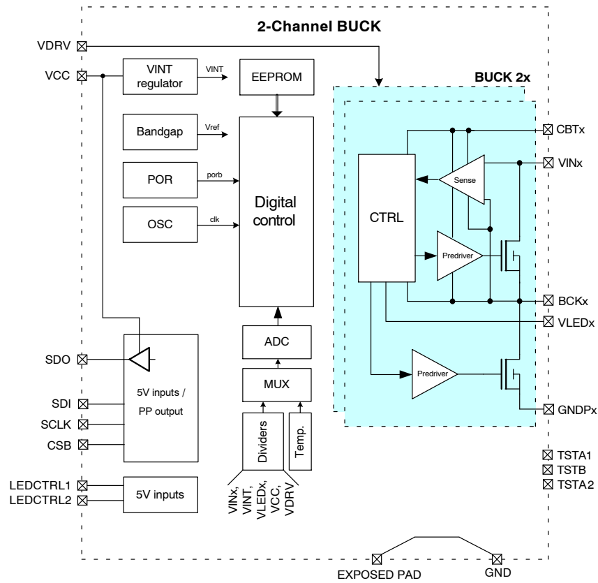
Figure 2. Block Diagram
