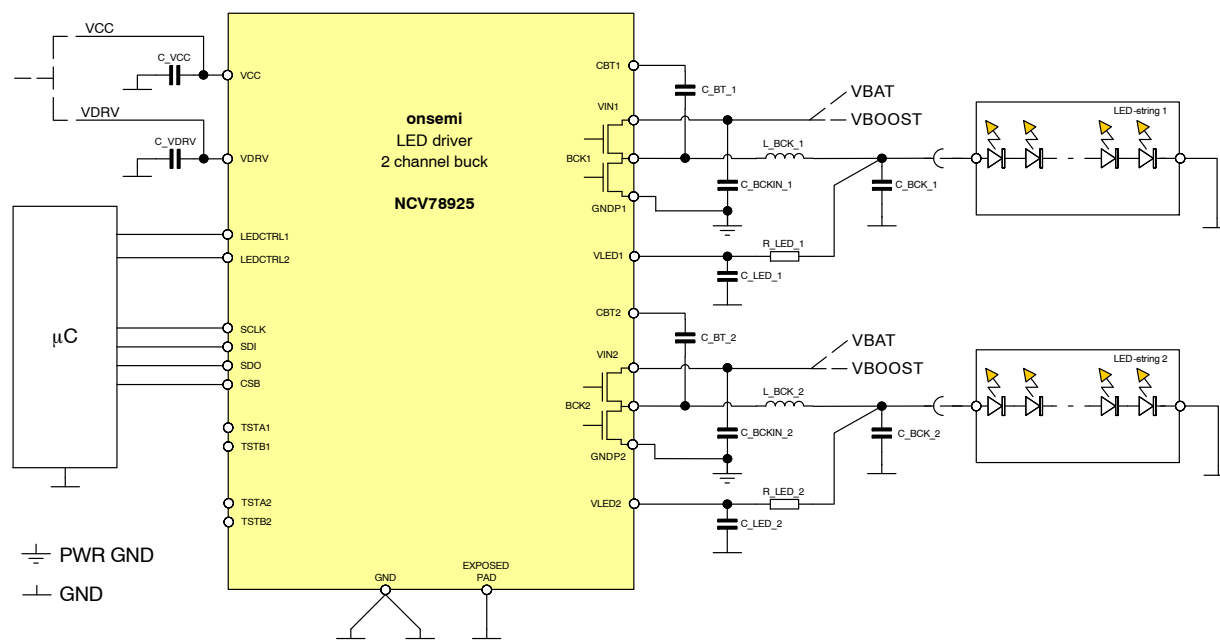
Figure 1. NCV78925 Typical Application Schematic
