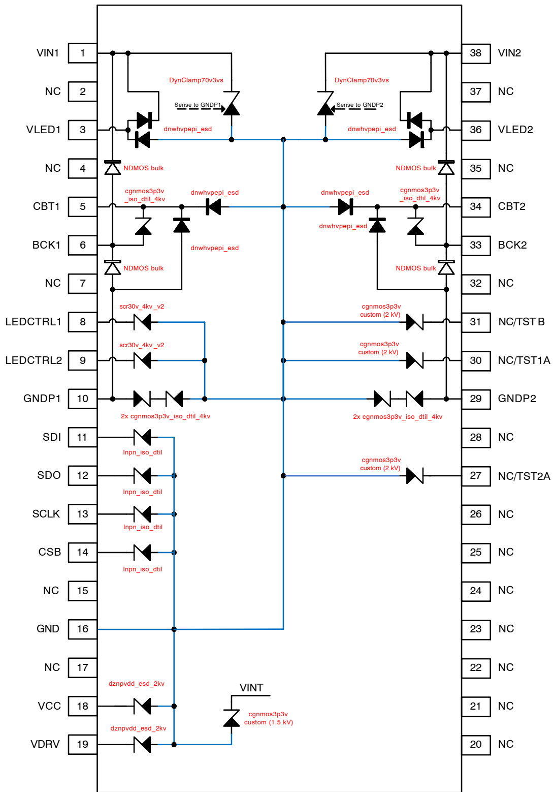
Figure 3. NCV78925 ESD Schematic
