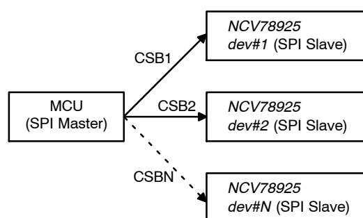
Figure 28. SPI Star Connection
