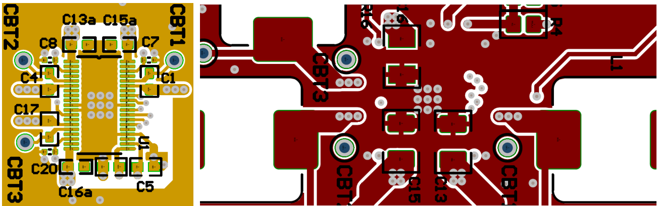
Figure 35. NCV78925/NCV78935 Top Side Exposed Pad Reference PCB Layout (Top and Bottom View)
