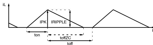
Figure 15. Inductor Current in DCM Mode
