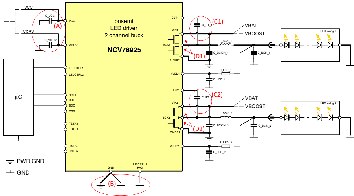
Figure 33. NCV78925 Application Critical PCB Areas
