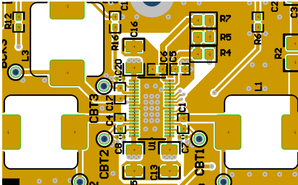
Figure 34. NCV78925/NCV78935 Bottom Side Exposed Pad Reference PCB Layout (Top View)
