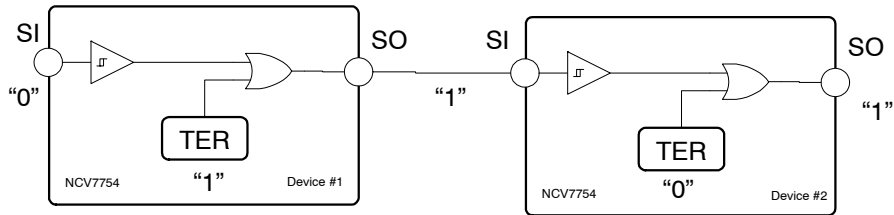
Figure 27. TCR Error Propagation
