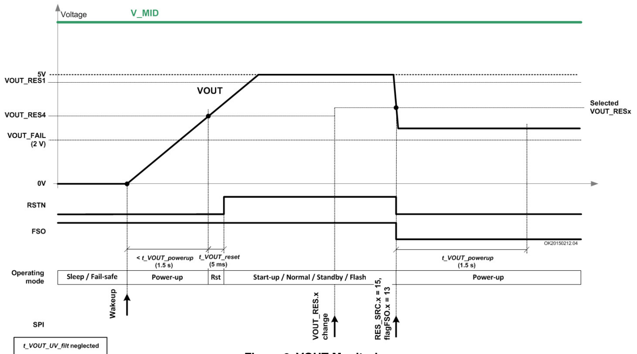
Figure 6. VOUT Monitoring
