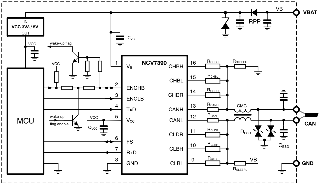
Figure 2. Typical Application Diagram with Sleep / Wake-up Mode
