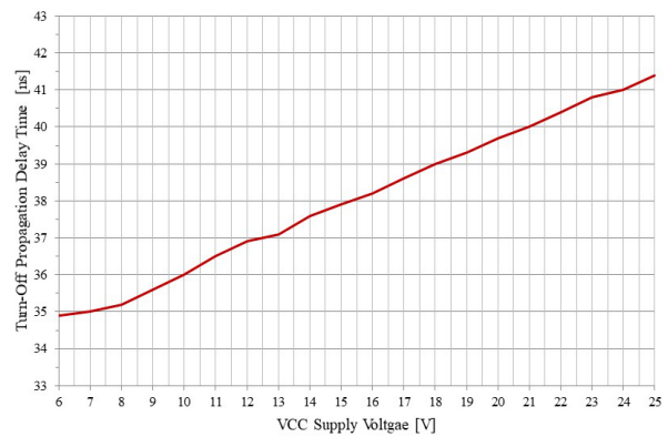
Figure 47. Turn-off Propagation Delay vs. V_{CC} Supply Voltage
