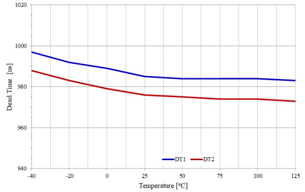
Figure 39. Dead Time vs. Temperature ( R_{DT} = 100\ k\Omega )
