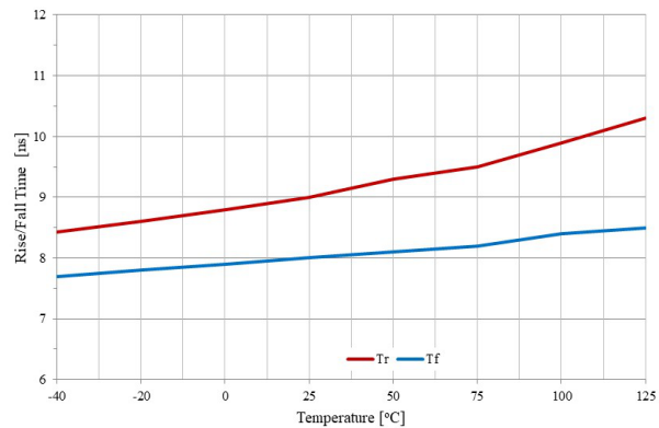
Figure 34. Rise/Fall Time vs. Temperature ( C_{LOAD} = 1.8 \text{ nF} )
