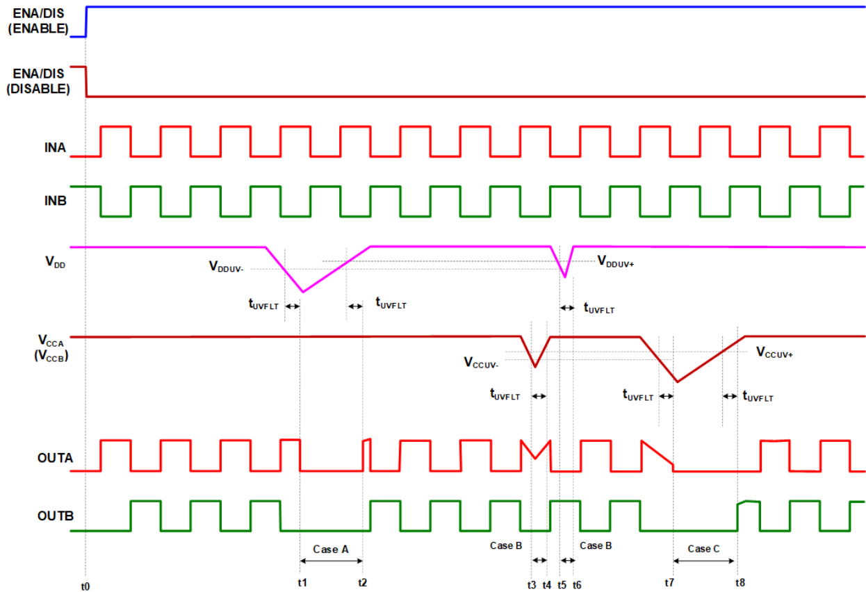
Figure 54. Timing Chart Under-Voltage Lockout Protection
