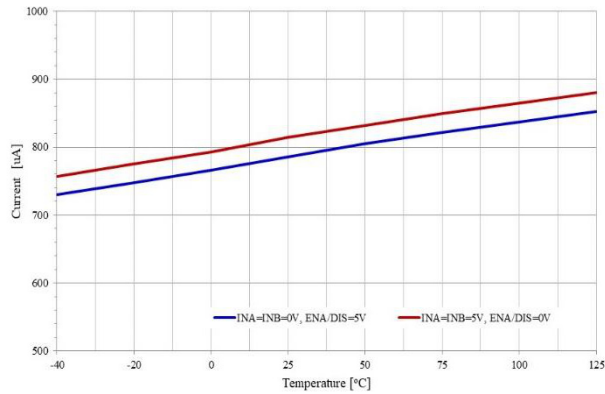
Figure 6. Quiescent V_{DD} Supply Current vs. Temperature ( V_{DD} = 5\text{ V} , I_{NA} = I_{NB} = 0\text{ V} , E_{NA}/DIS = 5\text{ V} or, I_{NA} = I_{NB} = 5\text{ V} , E_{NA}/DIS = 0\text{ V} and No Load)
