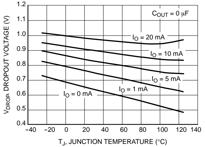
Figure 5. Dropout Voltage
