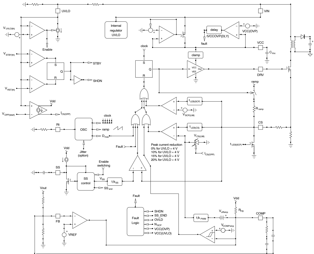
Figure 3. Block Diagram
