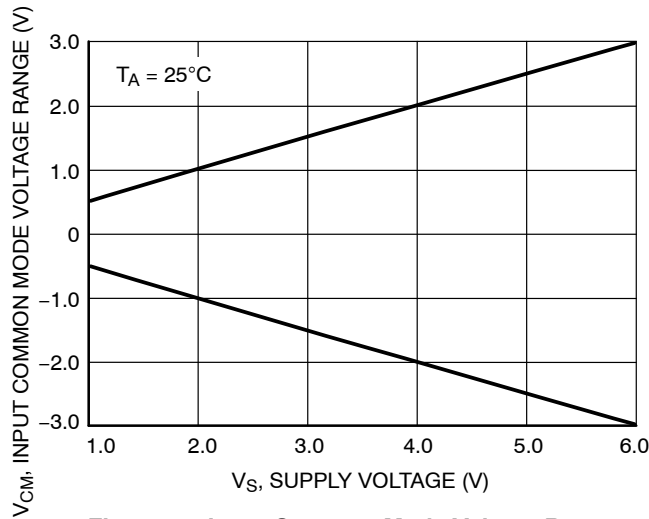
Figure 13. Input Common Mode Voltage Range versus Supply Voltage
