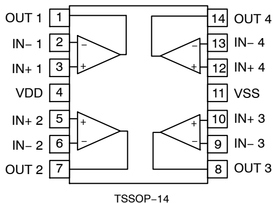
Quad Channel Configuration NCS21804
