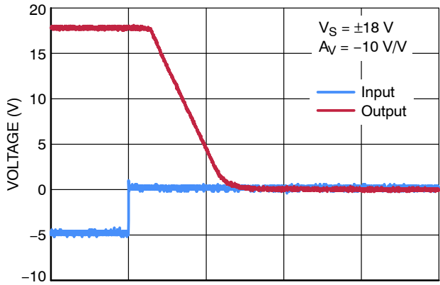
TIME (4 \mu\text{s}/\text{div} )
