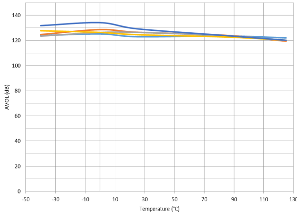
Figure 27. Open Loop Gain vs. Temperature, V S = 5.5 V
