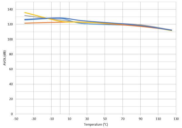
Figure 28. Open Loop Gain vs. Temperature, V S = 3 V
