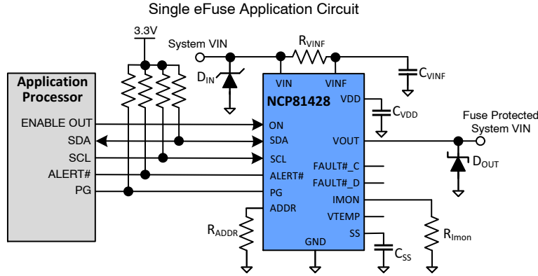
Figure 54. Application Circuit
