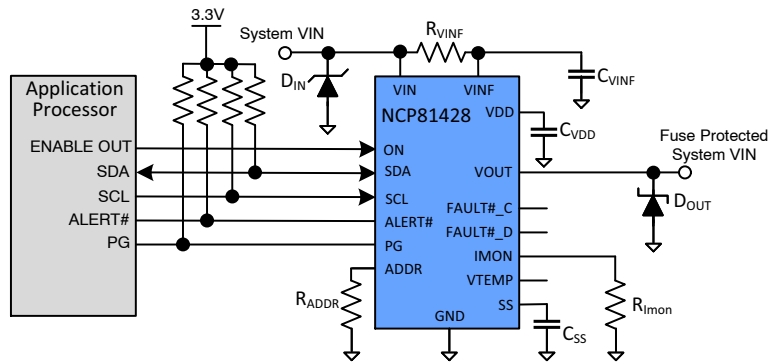
Figure 1. Application Schematic
