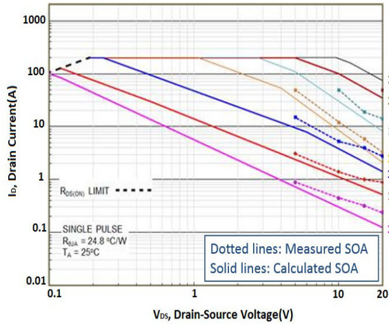
Figure 10. Power FETs Safe Operating Area
