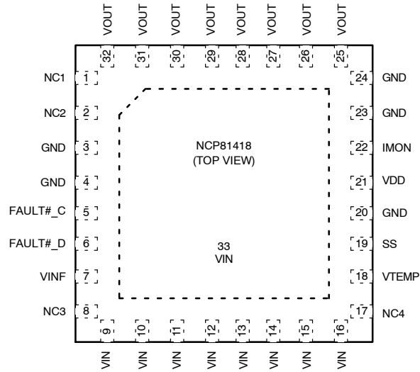
Figure 2. Pin Connections
