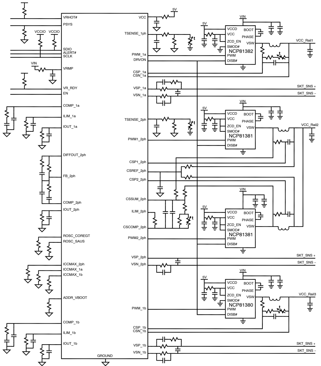
Figure 3. Application Schematic
