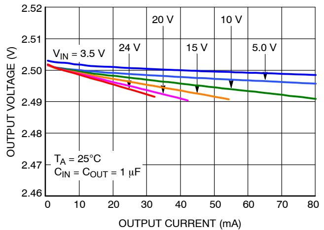
Figure 8. NCP716x25xxx Output Voltage vs. Output Current
