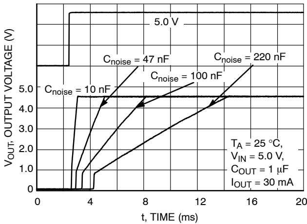
Figure 33. Turn-On Response
