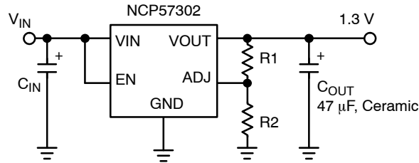
Figure 1. Adjustable Regulator
