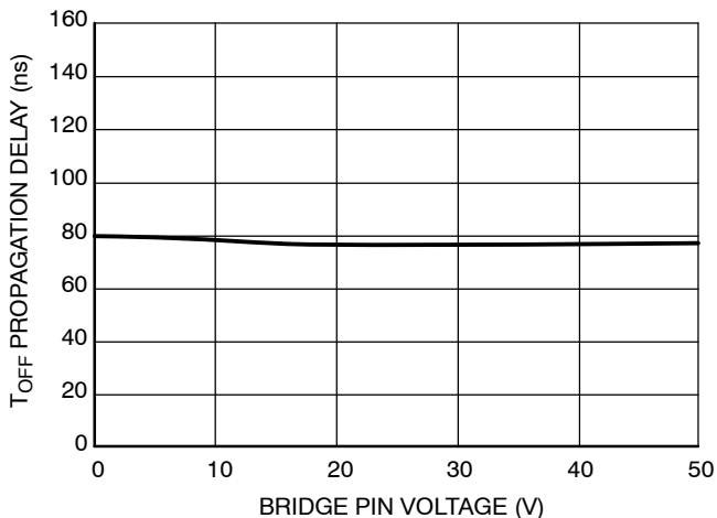
Figure 16. High Side Turn OFF Propagation Delay vs. V_{BRIDGE} Voltage
