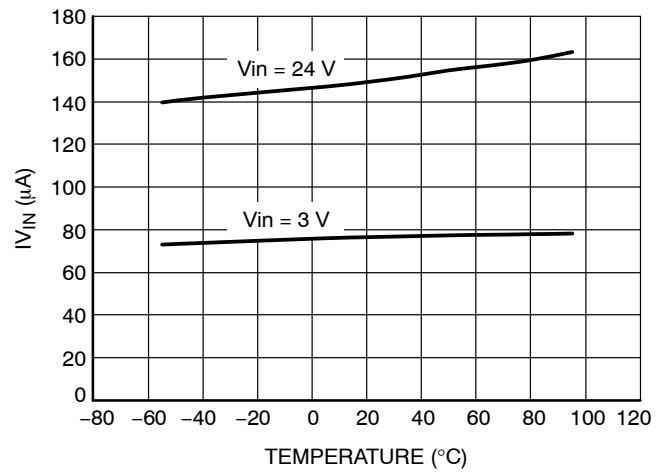
Figure 12. V_{in} Controller Current vs. Temperature ( EN = \text{HIGH} )
