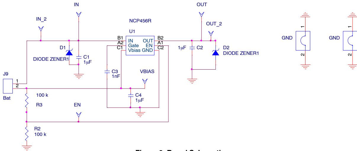
Figure 9. Board Schematic
