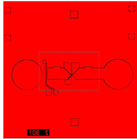
Figure 8. PCB Bottom View
