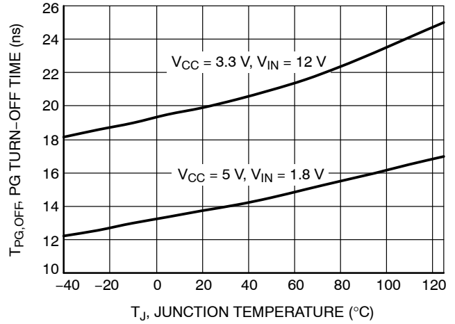
Figure 26. Power Good Turn-off Time vs. Temperature
