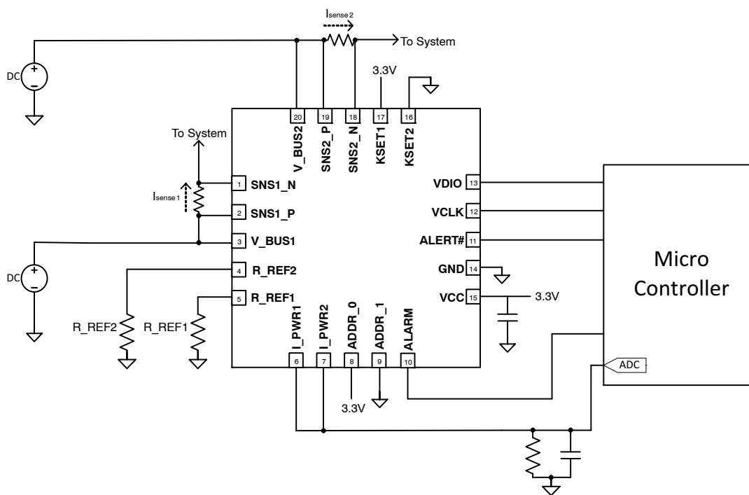
Figure 2. Application Schematic
