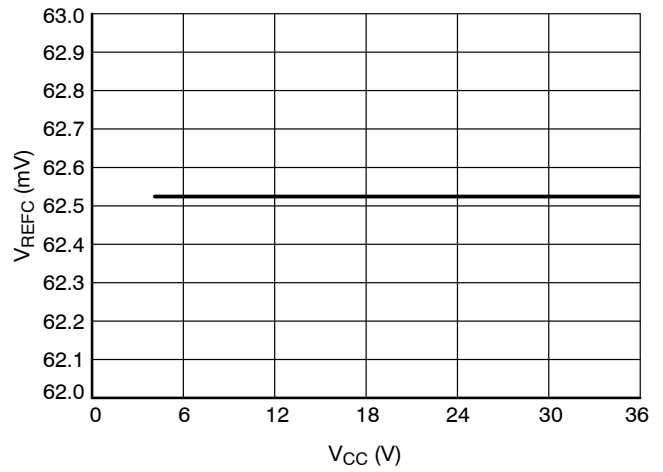
Figure 7. V_{REFC} at T_J = 25^\circ\text{C}
