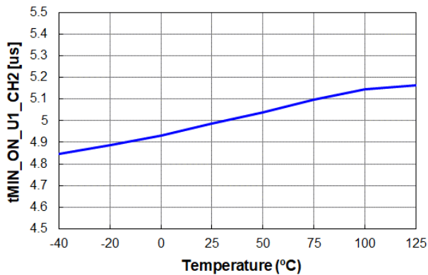
Figure 6. t_MIN-ON-U1-CH2 vs. Temperature
