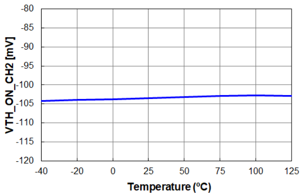
Figure 8. V_TH-ON-CH2 vs. Temperature
