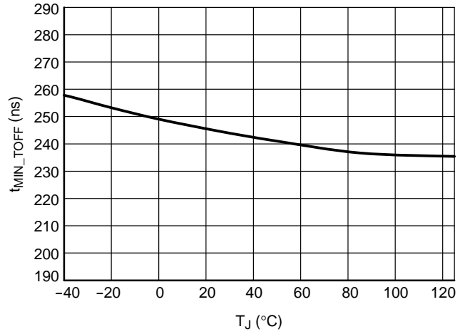
Figure 27. Minimum Off-time R_{MIN\_TOFF} = 0\ \Omega
