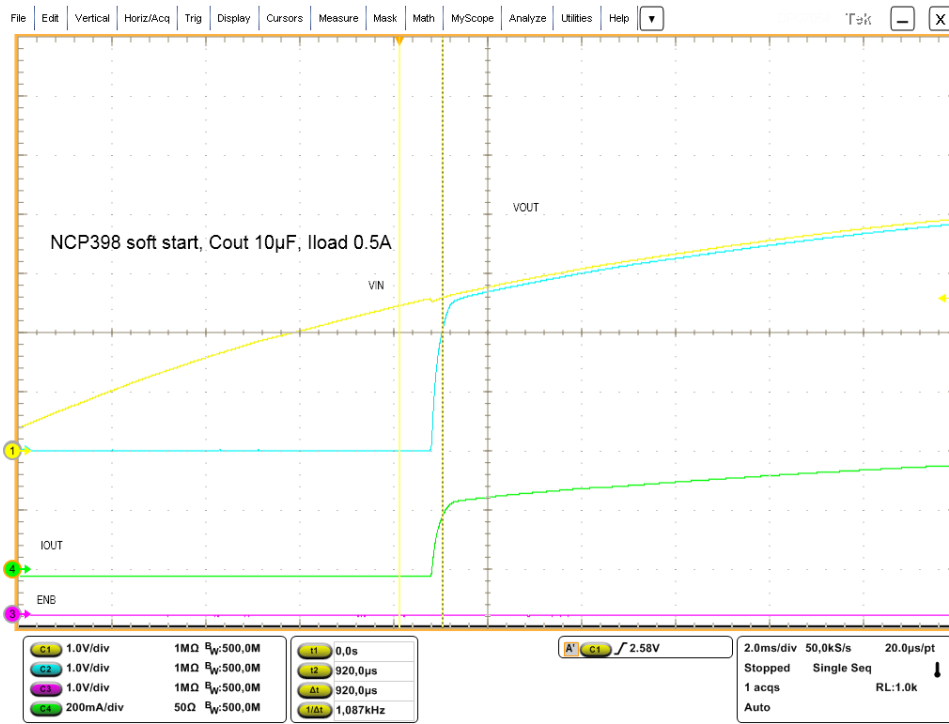
Figure 12. Soft Start On Cout 10 µF, 500 mA, Vin: yellow, Vout: blue, EN: pink, IOUT: green
