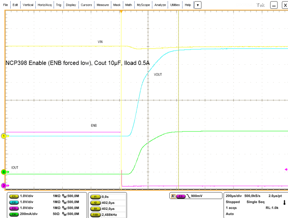
Figure 13. NCP398 Enable (ENB forced low) Vin: yellow, Vout: blue, EN: pink, IOUT: green
