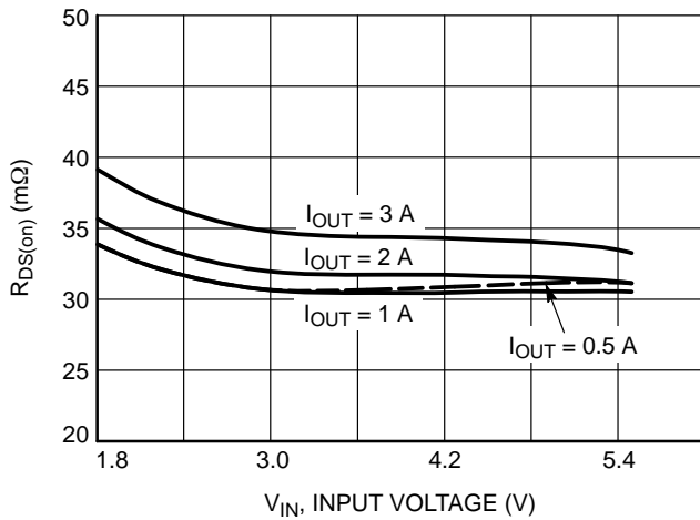
Figure 5. R_{DS(on)} vs. V_{IN} Voltage at 25\text{ }^\circ\text{C}
