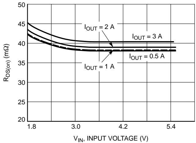
Figure 6. R_{DS(on)} vs. V_{IN} Voltage at 85\text{ }^\circ\text{C}
