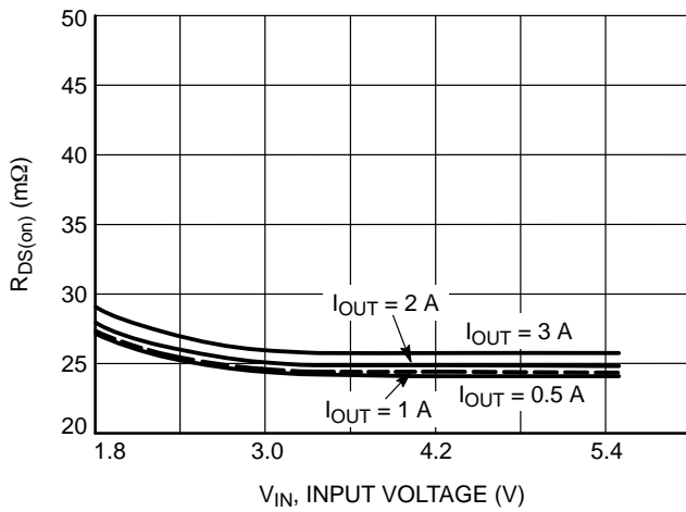
Figure 7. R_{DS(on)} vs. V_{IN} Voltage at -40\text{ }^\circ\text{C}
