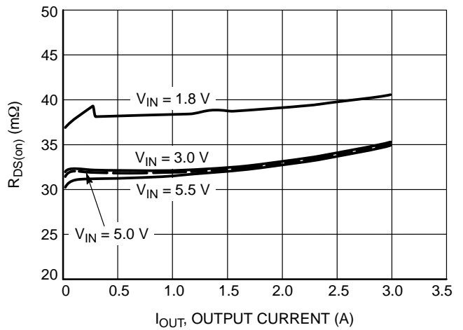
Figure 8. R_{DS(on)} vs. I_{OUT} at 25\text{ }^\circ\text{C}
