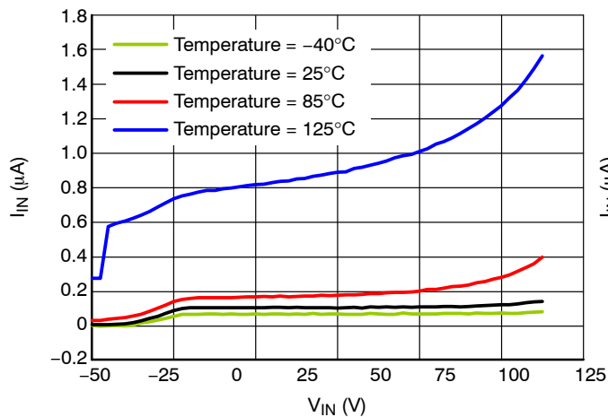
Figure 8. Standby Current (μA) versus V_{IN} (V), No Load
