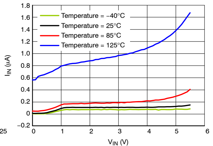
Figure 9. Standby Current (μA) versus V_{IN} (V), V_{OUT} Short to GND.
