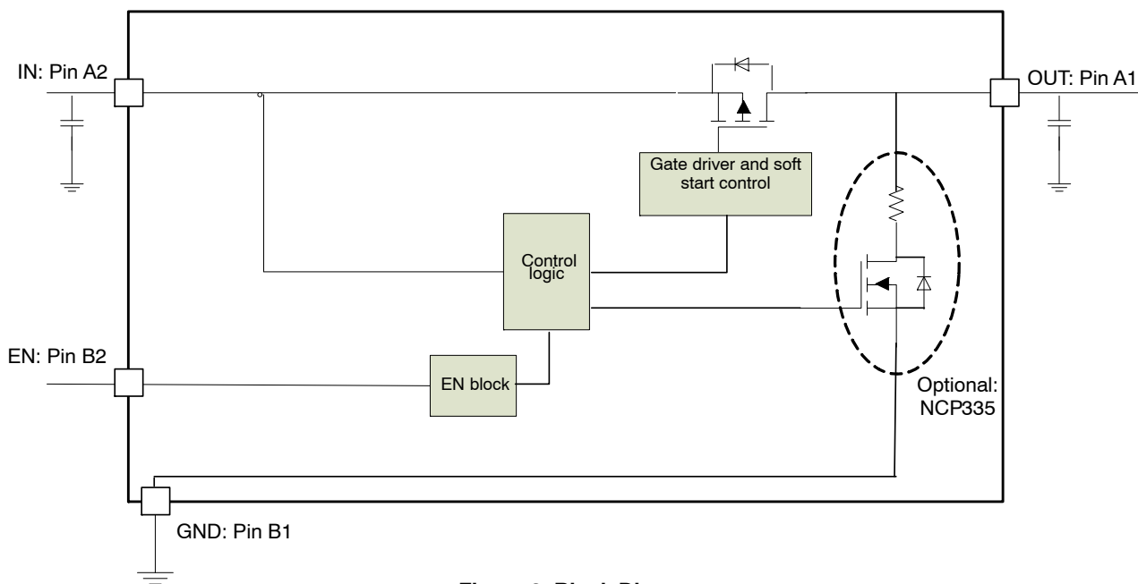
Figure 2. Block Diagram
