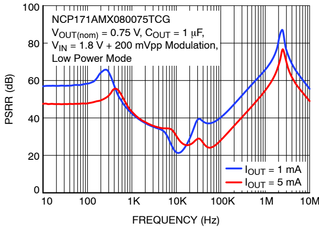
Figure 50. PSRR vs. Frequency in Low Power Mode
