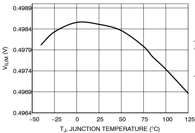
Figure 50. V_{ILIM} vs. Temperature
