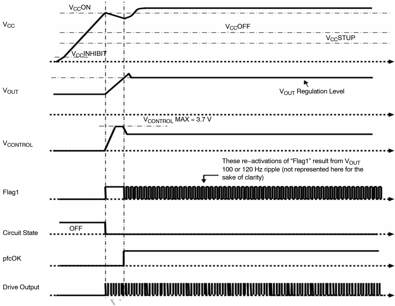
Figure 70. Startup Phase in Normal Conditions
