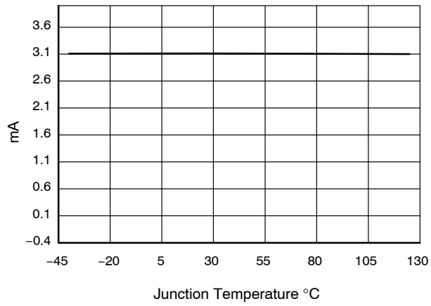
I_{CC3} ( I_{COMP} = 850\text{ }\mu\text{A} )
