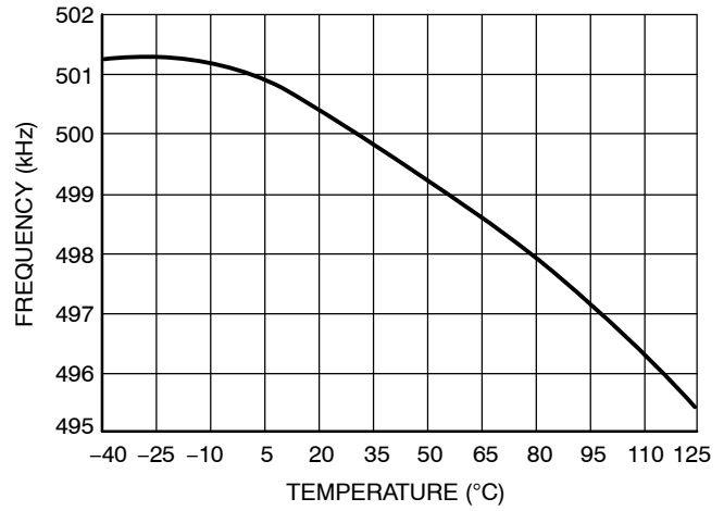
Figure 20. F_{sw \max}
