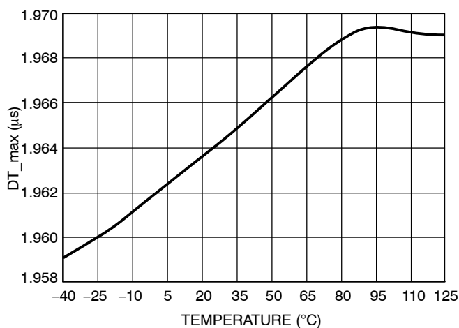
Figure 13. T_dead_max
