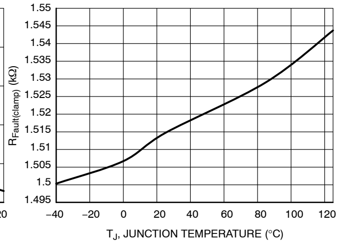
Figure 57. R Fault(clamp) vs. Temperature
