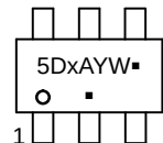
TSOP-6 (SOT23-6) SN SUFFIX CASE 318G STYLE 13
