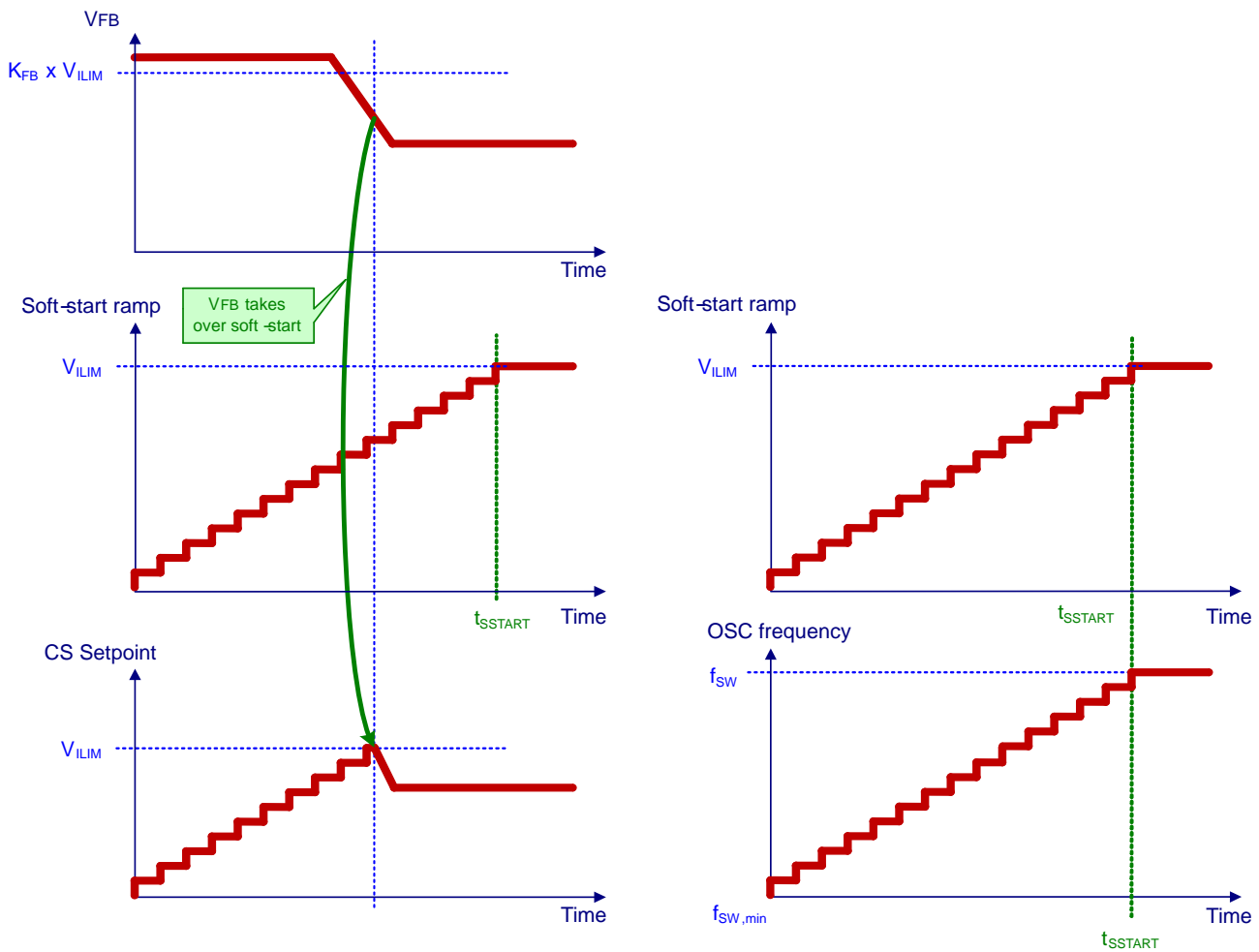
Figure 64. Soft-Start Feature
