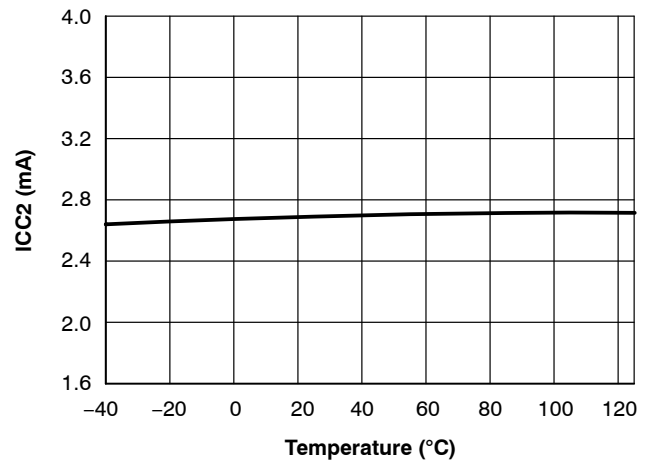
Figure 9. ICC2 (100-kHz Version) vs. Junction Temperature
