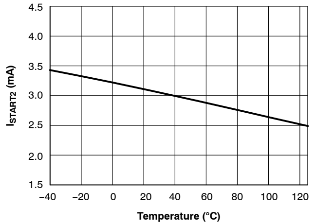
Figure 11. I START2 vs. Junction Temperature
