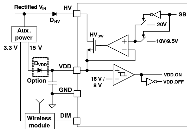
Figure 14. VDD Supply
