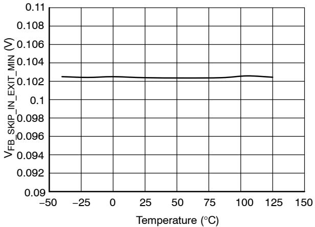
Figure 49. Minimum Voltage on the Skip Pin to Define the Skip in Level V_{FB\_SKIP\_IN\_EXIT\_MIN}
