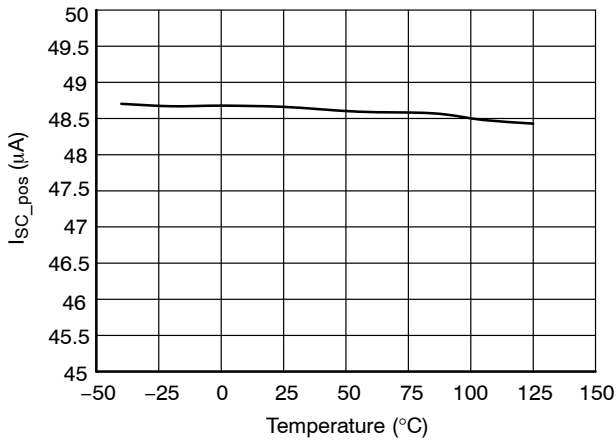
Figure 51. Current Sense Input Current I_{CS\_pos} @ V_{CS} = 3\text{ V}
