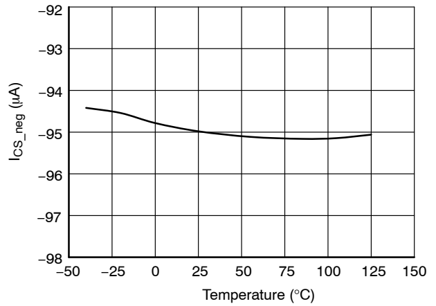
Figure 52. Current Sense Input Current I_{CS\_neg} @ V_{CS} = -3\text{ V}
