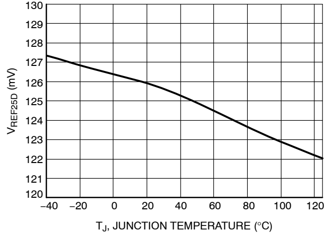
Figure 46. V_{REF25D} vs. Junction Temperature
