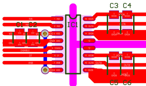
Figure 15. Recommended Layout (NCx57255, NCx57256)
